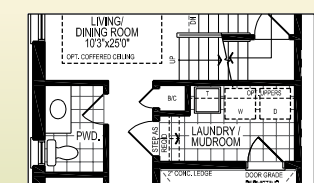
Partial Ground Floor Plan for Opt. Bed 2 Ensuite Elev. B1/B2 (Rev.)
