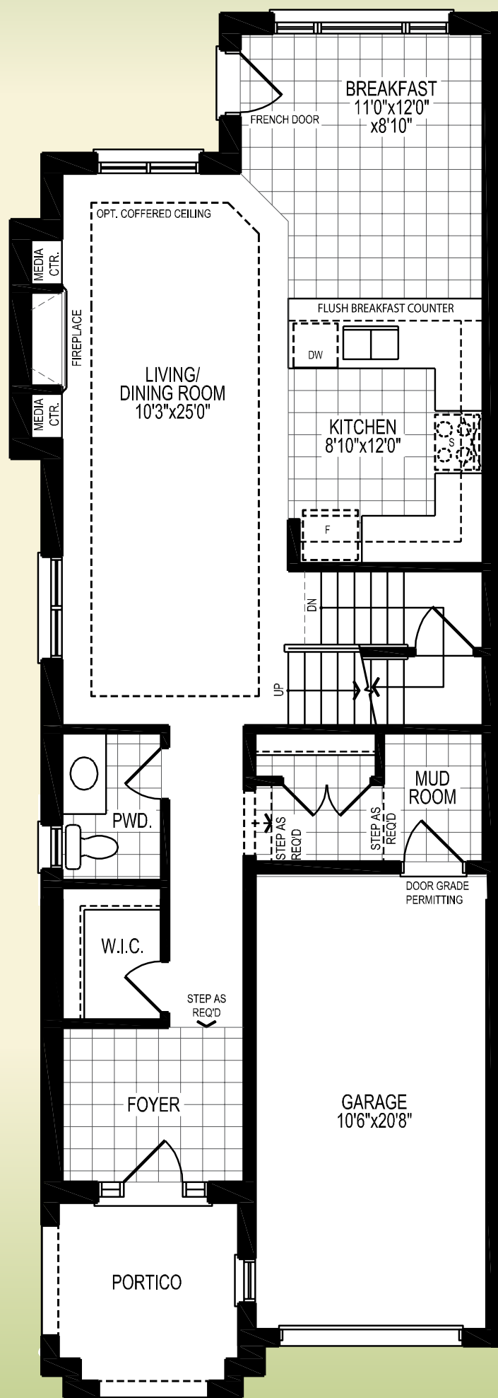
Ground Floor Plan Elev. B1
