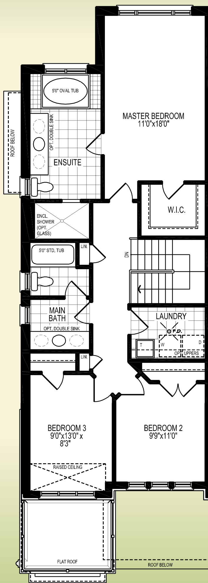
Second Floor Plan Elev. B1
