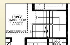
Partial Ground Floor Plan Opt. Finished Stairs to Basement & Landing Elev. B1/B2 (Rev.)
