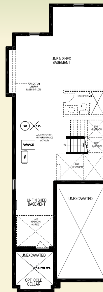
Basement Plan Elev. B1
