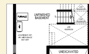
Partial Basement Plan for Opt. Bed 2 Ensuite Elev. B1/B2 (Rev.)
