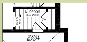
Partial Ground Floor Plan for Alternate Mudroom Elev. B
