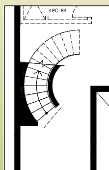
Partial Basement Plan for Opt. Curved Stairs to Basement
