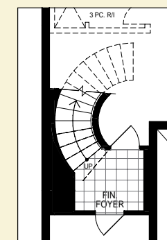
Partial Basement Plan for Opt. Open Curved Stairs to Basement
