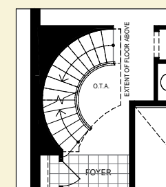
Partial Ground Floor Plan for Opt. Open Curved Stairs to Basement
