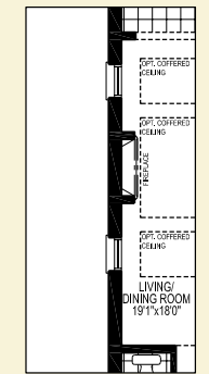
Partial Ground Floor Plan For Easement Lots Elev. B1/B2 (Rev.)
